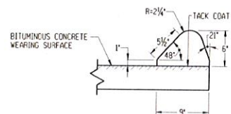
6" BITUMINOUS CONCRETE LIP CURBING
