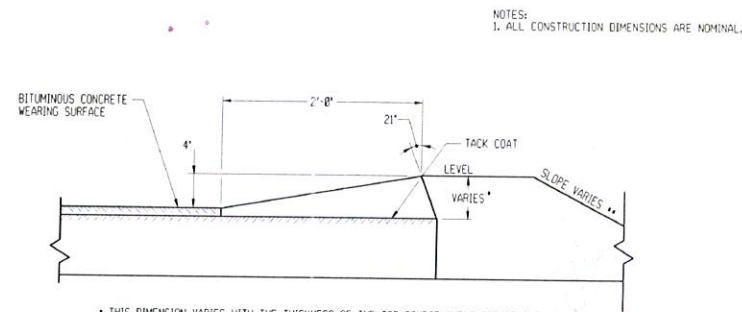
BITUMINOUS CONCRETE BERM
