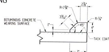
4" BITUMINOUS CONCRETE PARK CURBING
