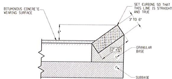
TYPICAL SECTION SHOWING SLOPE CURBING SET ADJACENT TO BITUMINOUS CONCRETE SURFACES
