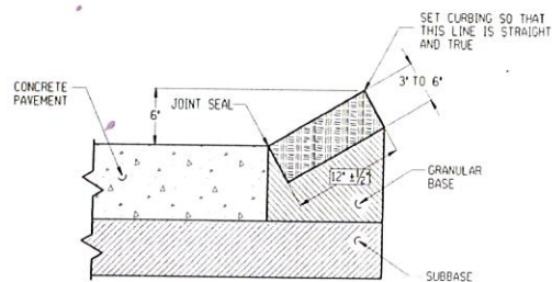
TYPICAL SECTION SHOWING SLOPE CURBING SET ADJACENT TO CONCRETE SURFACES
